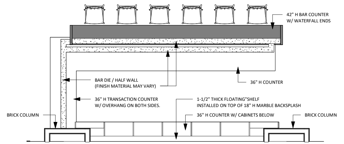
② Proposed - Level 1 - Bar Detail 1/4" = 1'-0"
