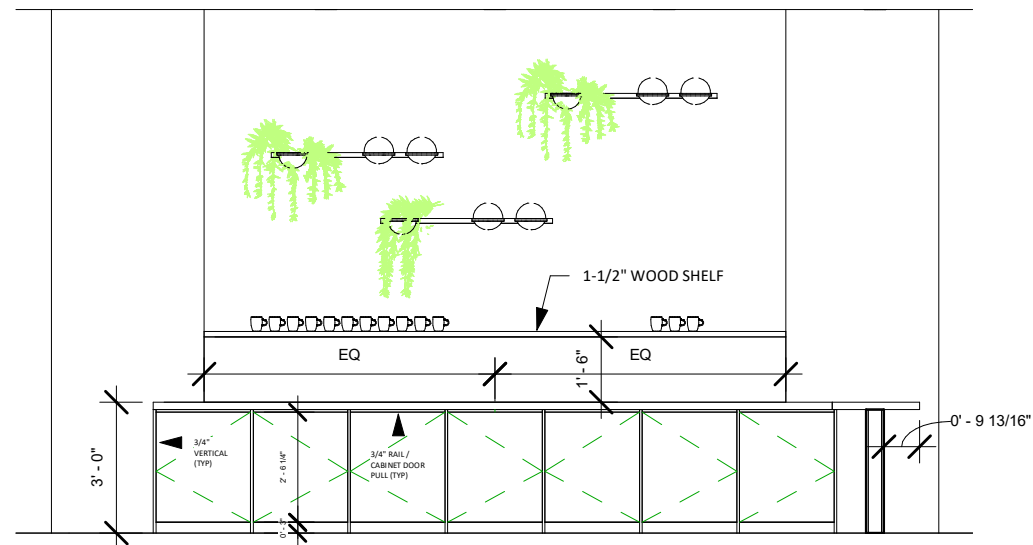
① ELV 2 1/4" = 1'-0"
