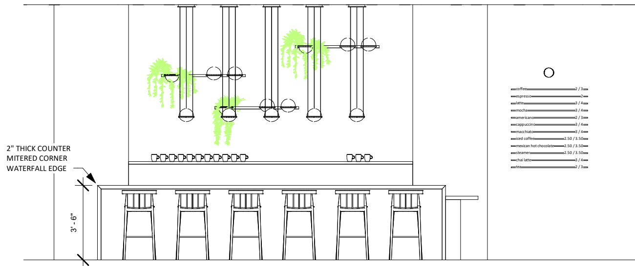
③ ELV 1 1/4" = 1'-0"
