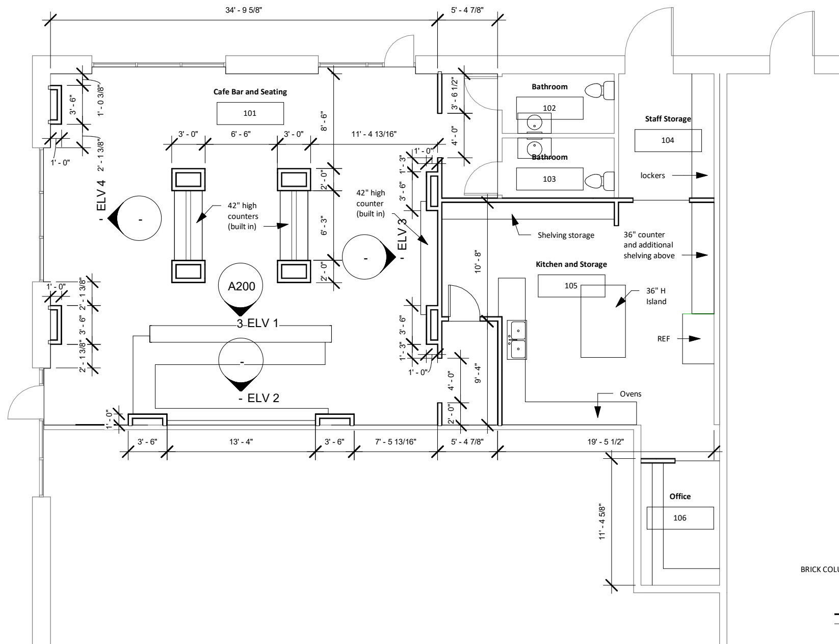
① Proposed - Level 1 (NO FURN) 1/8" = 1'-0"
