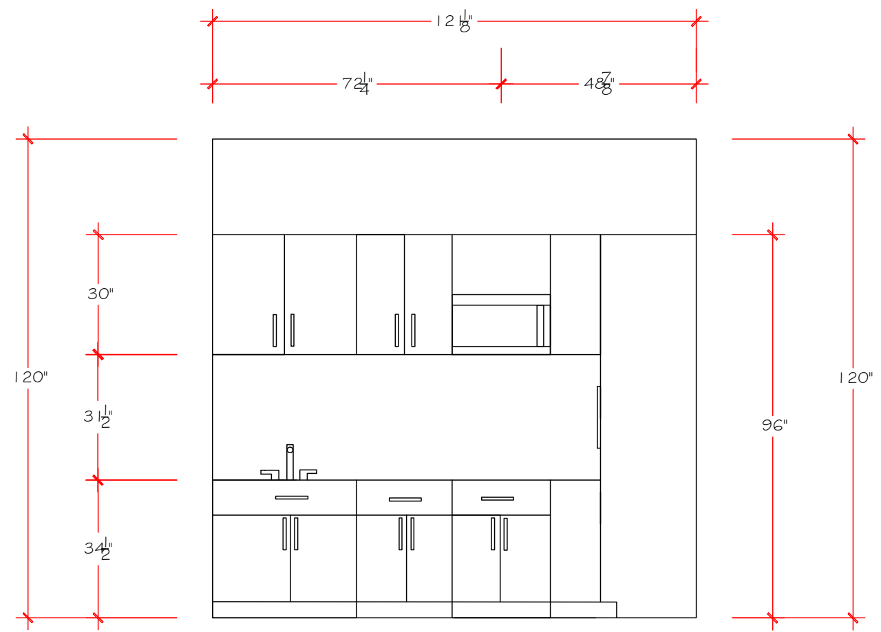
2 KITCHEN ELEVATION
