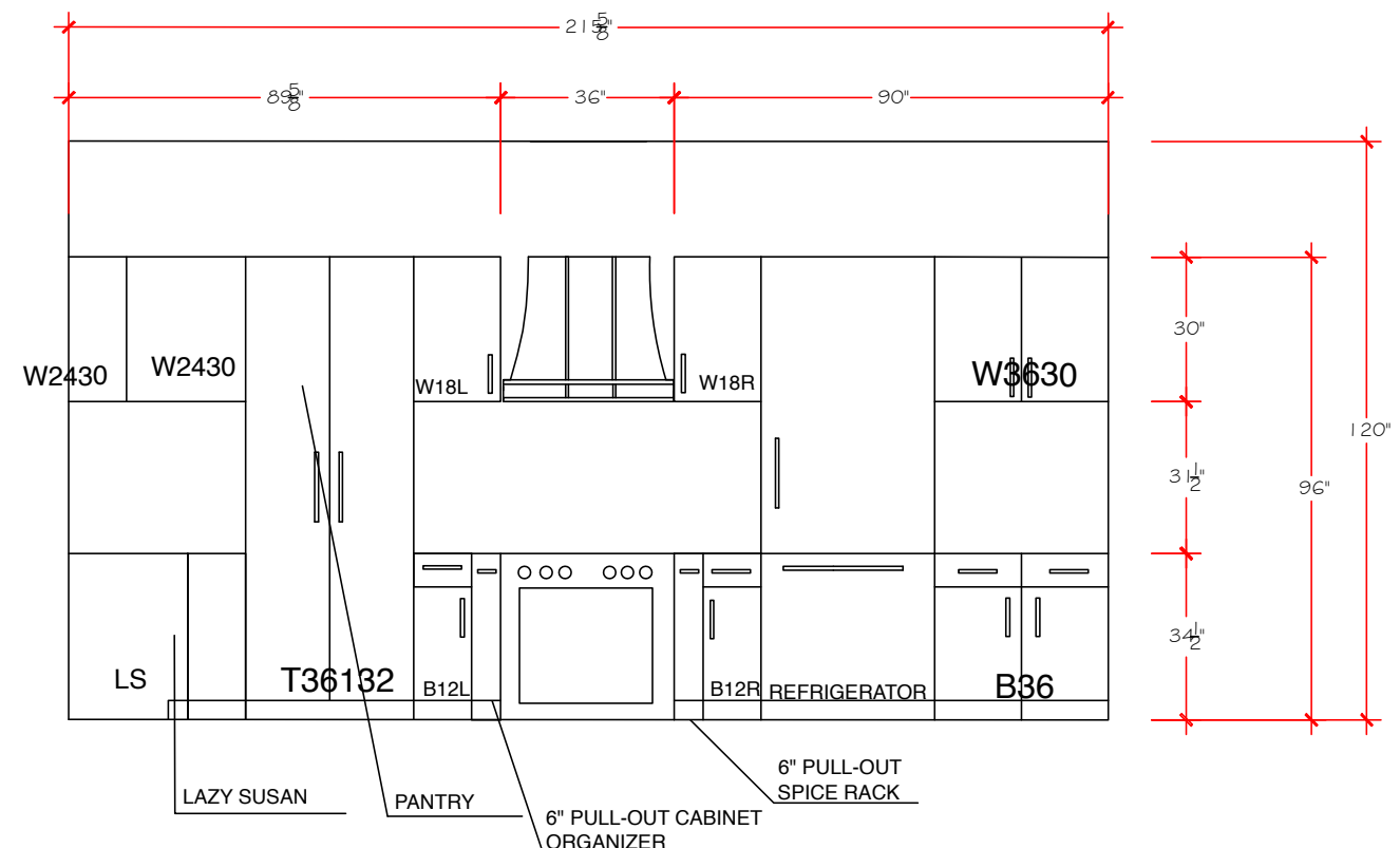
1 KITCHEN RANGE WALL ELEVATION
