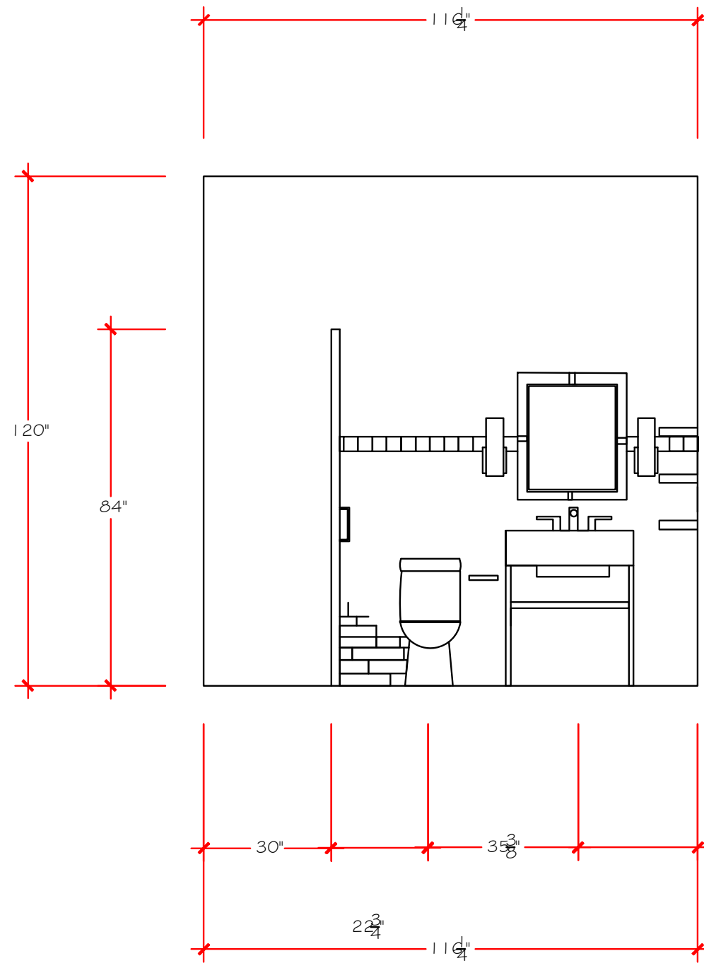
3 BATHROOM ELEVATION
