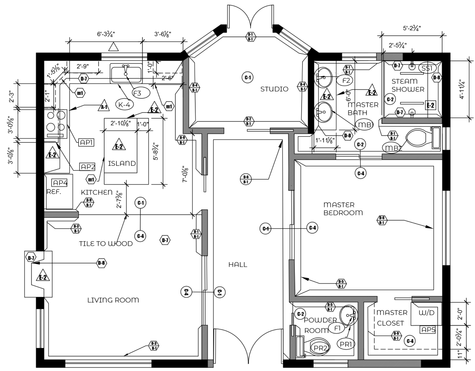
JOHNSON FINISH PLAN Scale: 1/4" = 1'-0" CLAUDIA FOLK WRIGHT
