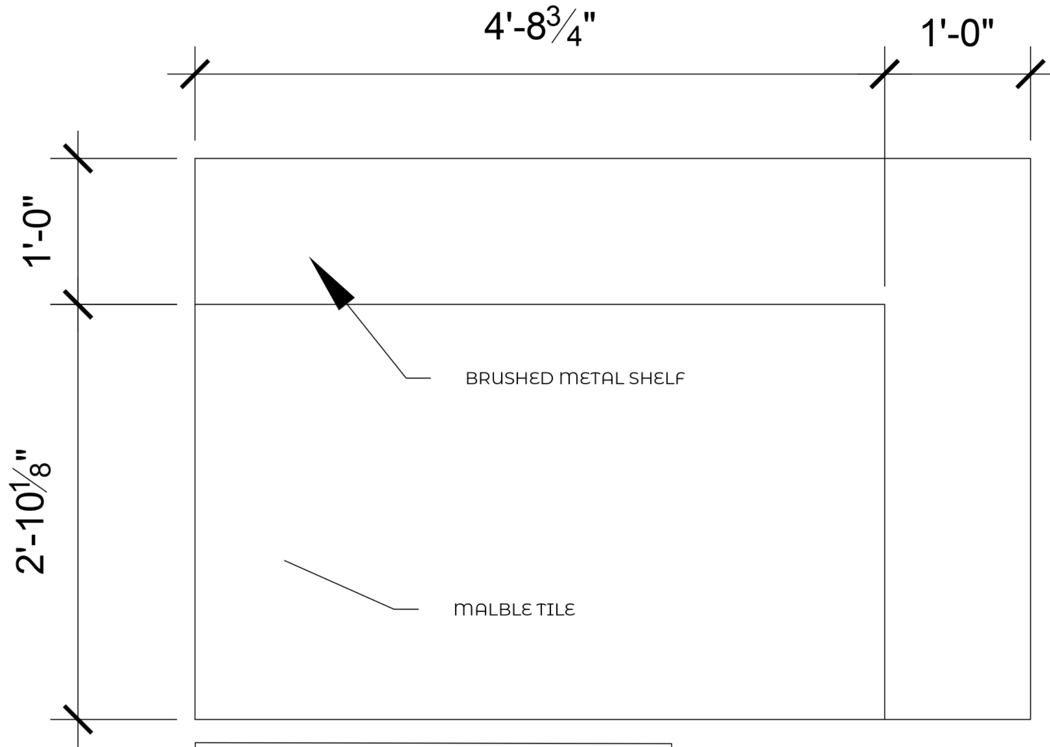
1 ISLAND DETAIL PLAN VIEW A5.1 Scale: 1-1/2"=1'-0" CLAUDIA FOLK WRIGHT
